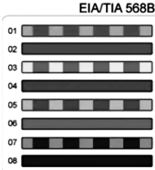
Guias do conector RJ45
